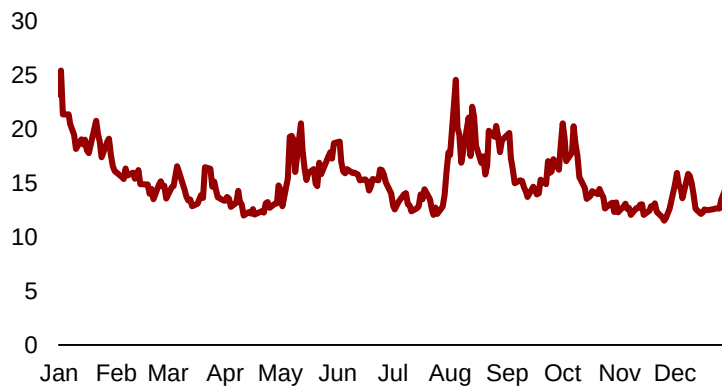
Figure 5: 2019 VIX Index
